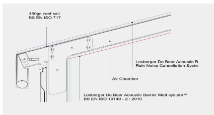
Acoustic roof detail
