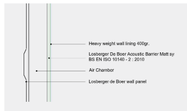
Acoustic wall detail
